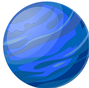
Neptune
